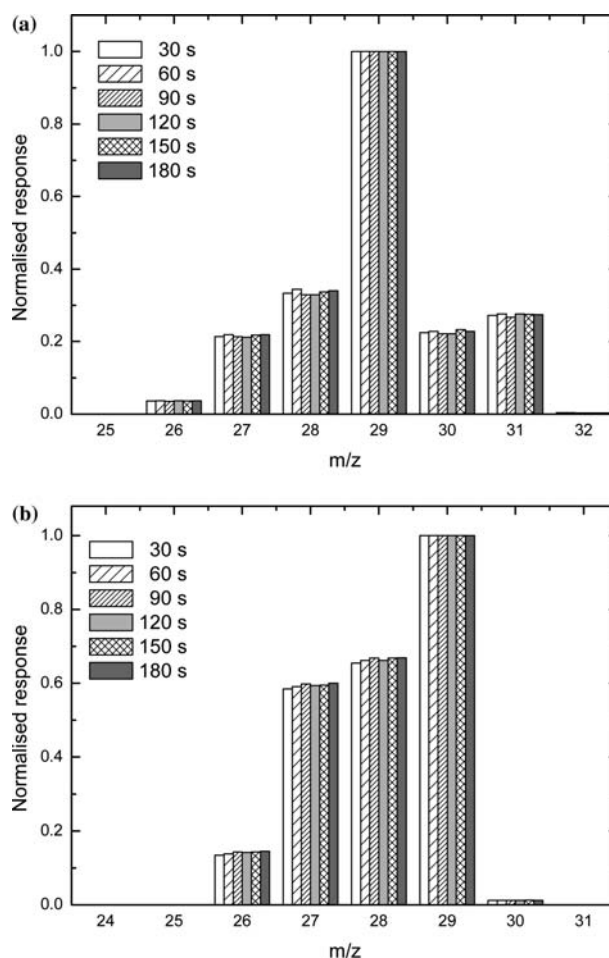
Figure 5. Mass fragmentation pattern of (a) ethane and (b) ethene in the reactor effluent after switching the gas feed from ^{12}\text{C}-\text{C}_2\text{H}_6/\text{He} via He to 1-^{13}\text{C}-\text{C}_2\text{H}_6/\text{He} over a 13wt% \text{Cr}/\text{Al}_2\text{O}_3 catalyst (200 mg) at 580 °C, 1 atm, with gas feed composition \text{C}_2\text{H}_6 : He = 2:20 (Nml/min).
