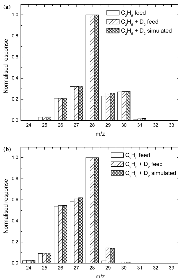
Figure 3. Mass fragmentation pattern of (a) ethane and (b) ethene in the reactor effluent during a dehydrogenation experiment with gas feed composition \text{C}_2\text{H}_6:\text{D}_2:\text{He}=2:0:20 or 2:1:20 (Nml/min). Test conditions: 13 wt% \text{Cr}/\text{Al}_2\text{O}_3 catalyst (200 mg), 580 °C, 1 atm.
