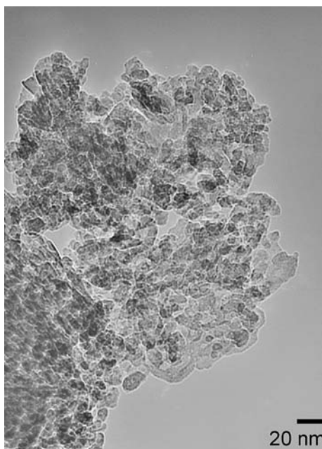
Figure 6. TEM micrograph ( \times 200 k) of used 13 wt% Cr/ \text{Al}_2\text{O}_3 catalyst showing alumina agglomerates with Cr-oxide particles.
