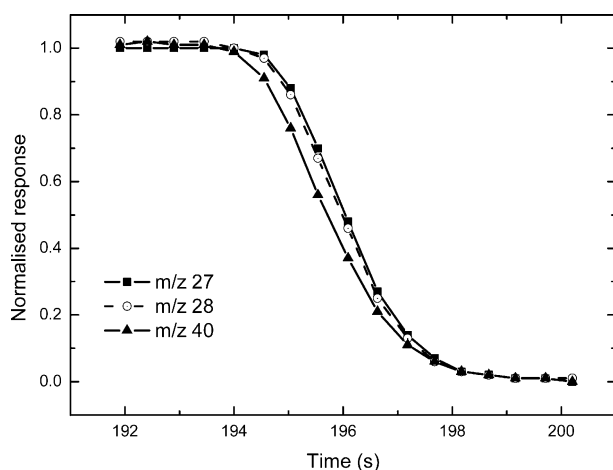
Figure 4. Transient responses observed in the reactor effluent when switching from a \text{C}_2\text{H}_6:\text{Ar}:\text{He}=2:1:20 (Nml/min) to a \text{Ne}:\text{He}=3:20 (Nml/min) feed over a 13 wt% \text{Cr}/\text{Al}_2\text{O}_3 catalyst (200 mg) at 580 °C, 1 atm. m/z 40 is characteristic of Ar.
