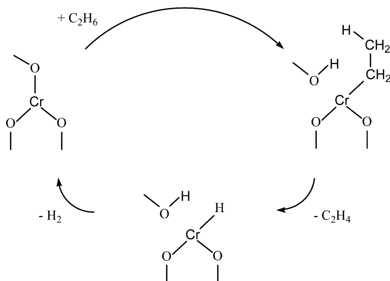
Figure 1. Schematic reaction mechanism for the dehydrogenation of alkanes over a \text{Cr}^{3+}\text{-O} active site.
